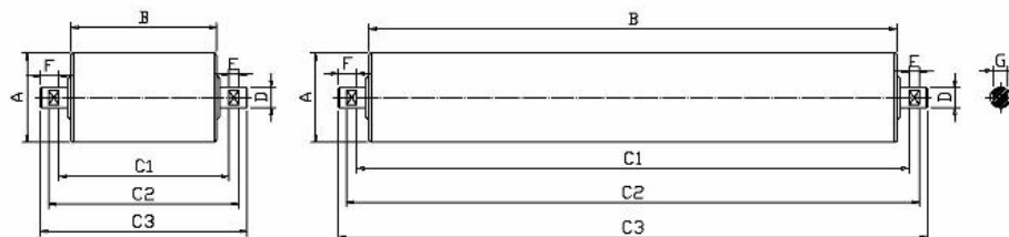
center roller
