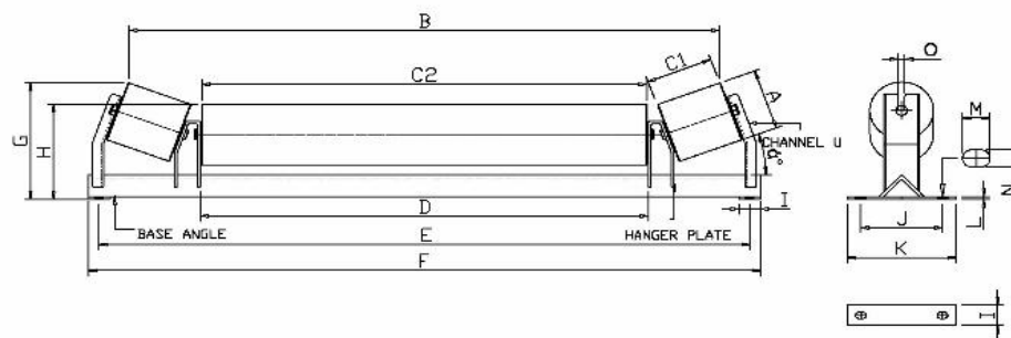
center roller
